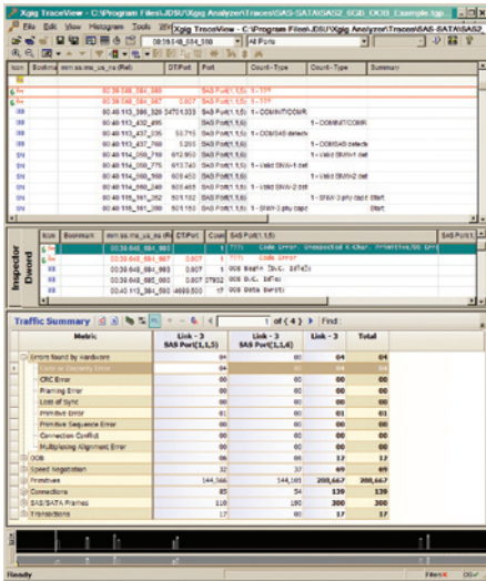
Figure 1: Xgig TraceView with new Trace Summary View (TSV)
